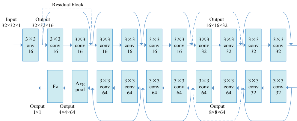
Fig. 1. Deep residual network model.
