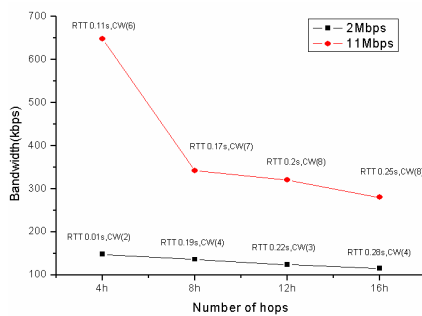
Fig. 9. Measured bandwidth and RTT
