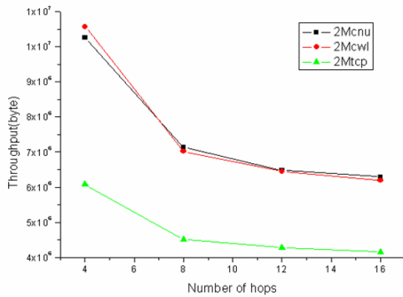
Fig. 7. TCP throughput on the 2Mbps link topology
