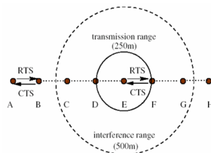
Fig. 1. Hidden-terminal problem
