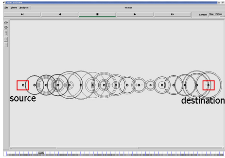
Fig. 6. Simulation topology
