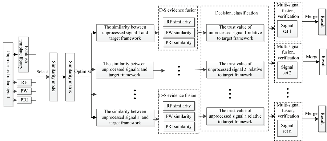
Fig. 6. Algorithm flow.
