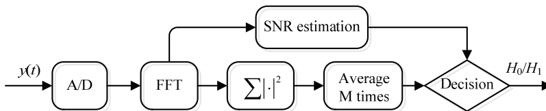
Fig. 3. Block diagram of adaptive double threshold ED.
