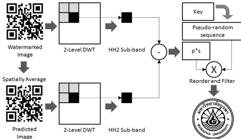
Fig. 4. A diagram outlining the proposed extraction process.
