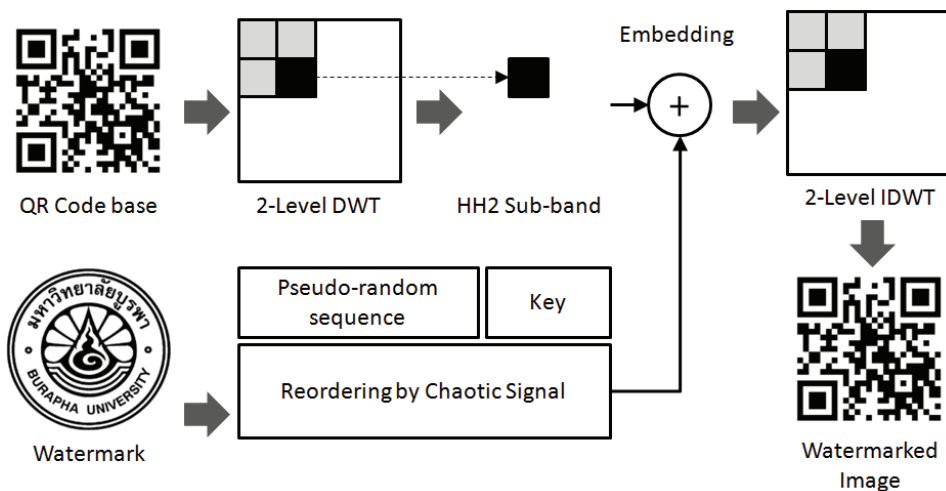
Fig. 2. A diagram outlining the proposed embedding process.
