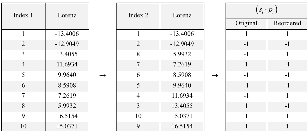
Fig. 3. An example of Lorenz calculation (left), sorted index (middle) and re-ordered watermark and pseudo-random sequences (right).
