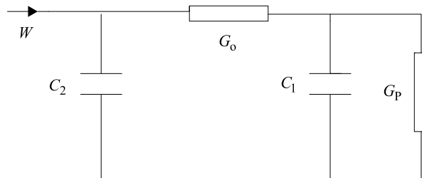
Fig. 2. Equivalent network of high voltage power cable.
