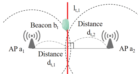
Fig. 2. Two circles are overlapped by two points.
