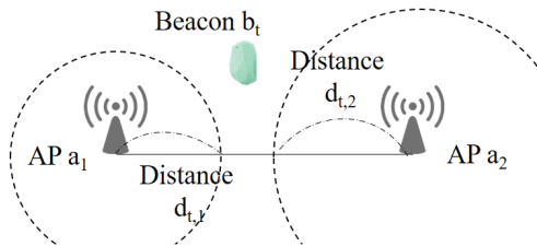
Fig. 5. Two circles in trilateration are not overlapped.
