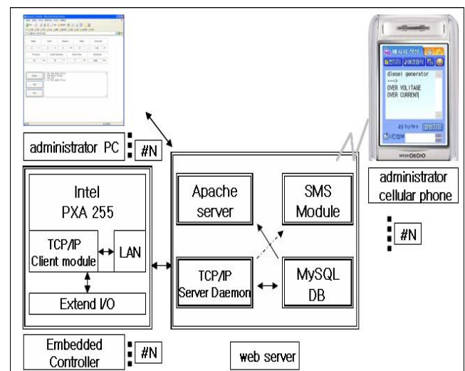
Fig. 1. Entire system block diagram
