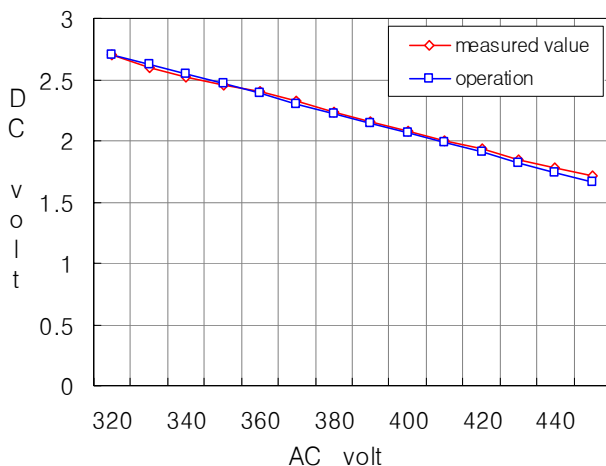
Fig. 8. Transformed DC voltage from generated AC voltage
