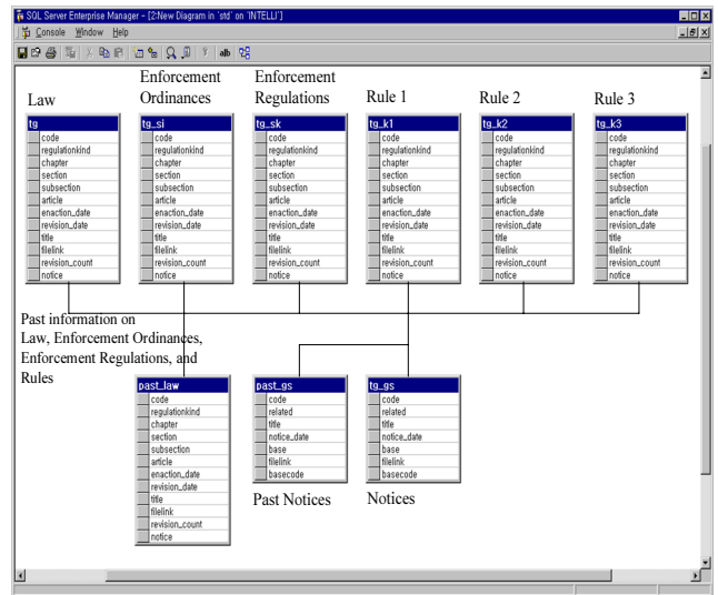
Fig. 5. Database schema of the Information System
