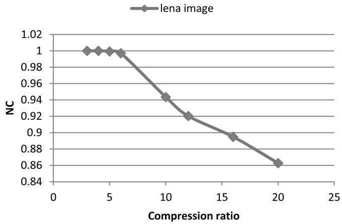
Fig. 13. Compression ratio vs. normalization correlation (NC).
