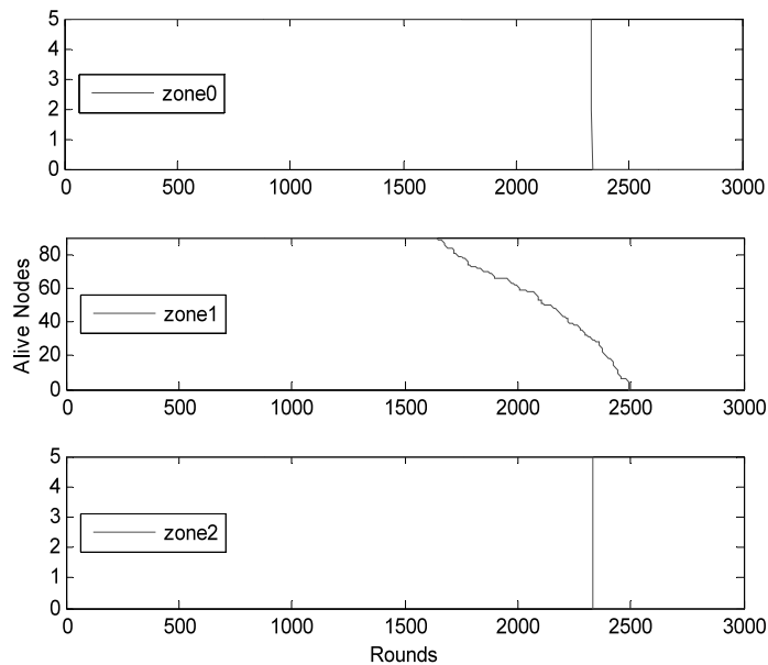
Fig. 11. Nodes distribution in network.
