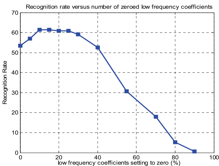
Fig. 9. Recognition rate versus number of zeroed low frequency coefficients.
