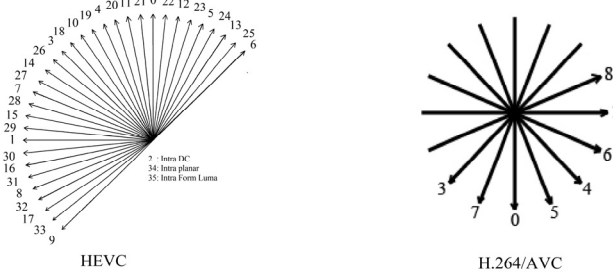
Fig. 1. Comparison between H.264 Advanced Video Coding (H.264/AVC) and High Efficiency Video Coding (HEVC) intra prediction directions.
