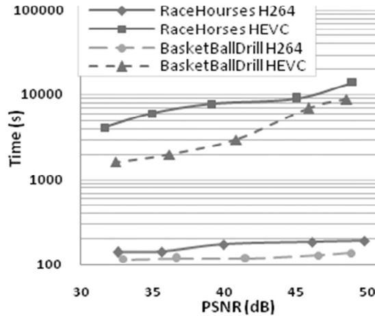
Fig. 7. Comparison of the fluctuation of encoding time with average PSNR for Class C sequences. PSNR=peak signal-to-noise ratio, HEVC=High Efficiency Video Coding.
