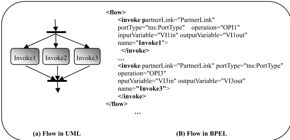
Fig. 11. The flow activity. UML=unified modeling language, BPEL=business process execution language.
