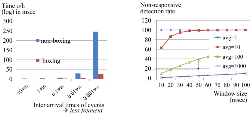
Fig. 5. (a) Time overhead according to inter event times, and (b) Non-responsive detection rates according to window sizes 0
